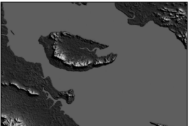
MODELO DIGITAL DE RELIEVE, Hoja Berrugate; Relieve sombreado SRTM Level 1 (3-arc sec)
